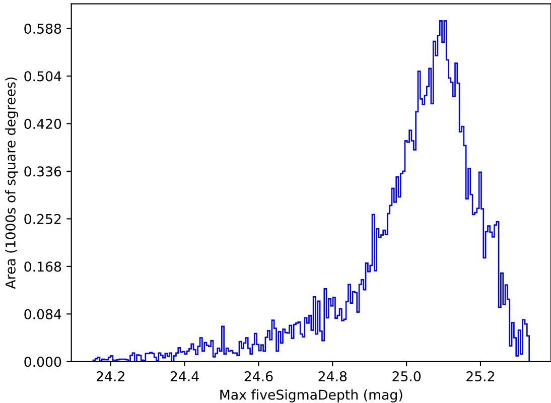
weather_cloudso0v3.5_10yrs All sky all bands: Max fiveSigmaDepth
