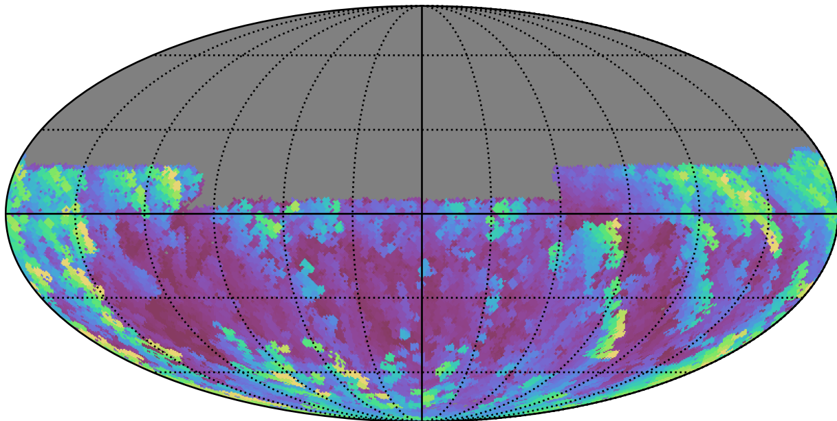
weather_cloudso0v3.5_10yrs Yr 1 y band: Max airmass
