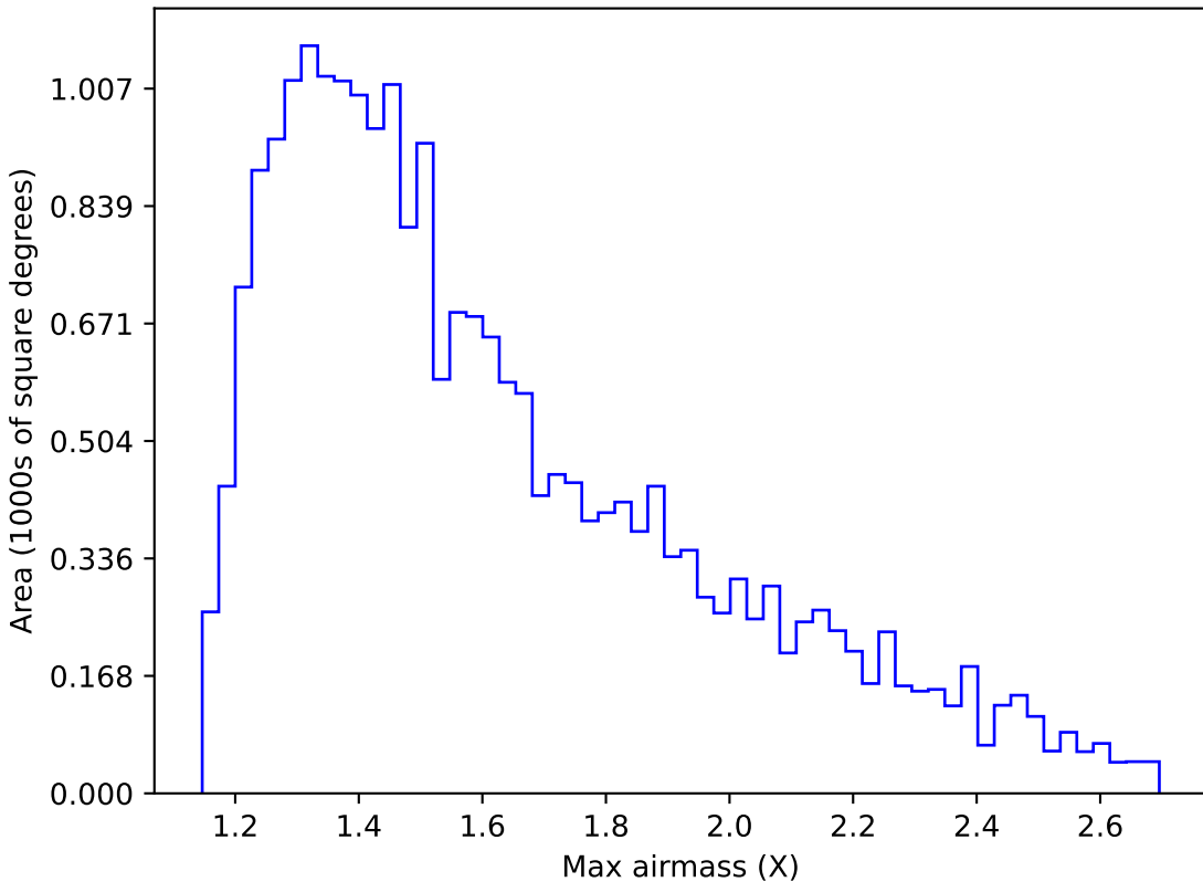
weather_cloudso0v3.5_10yrs Yr 1 y band: Max airmass
