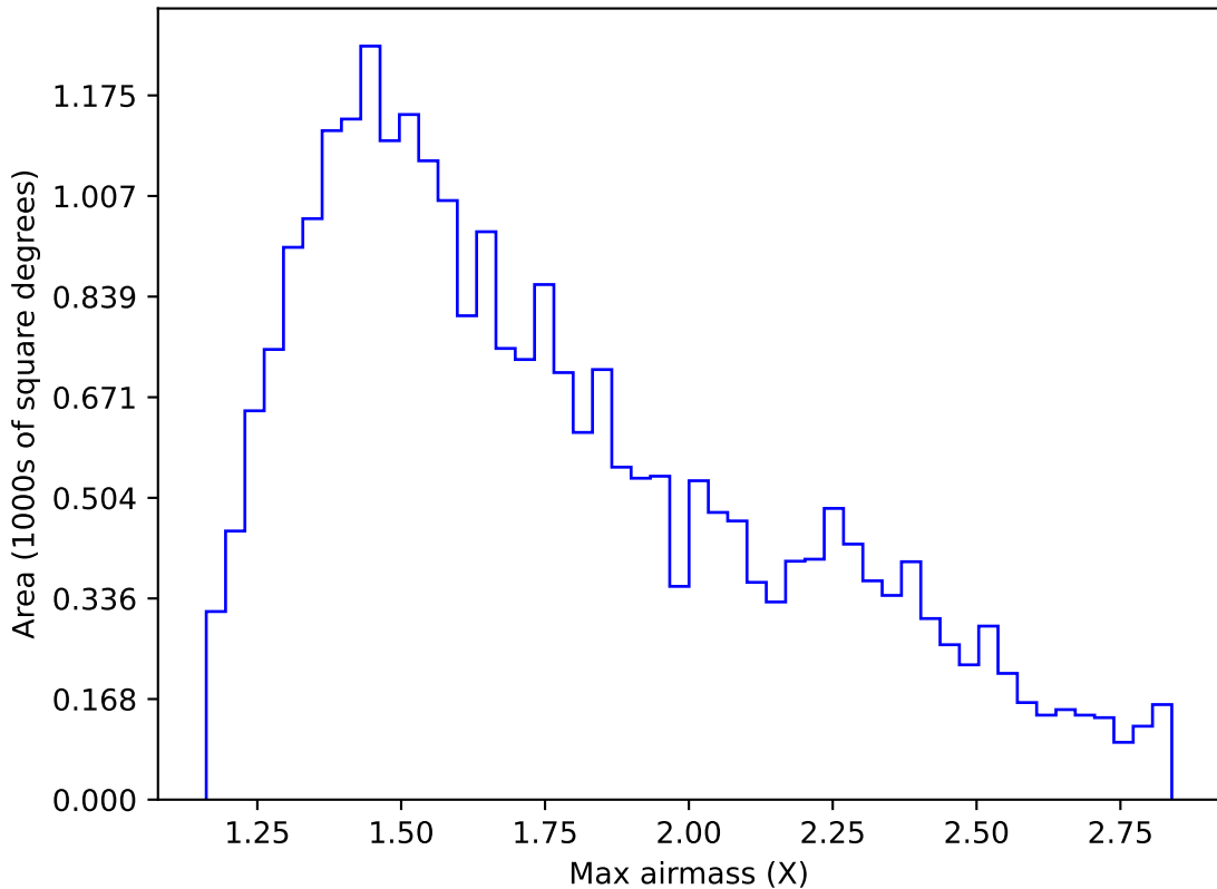
weather_cloudso0v3.5_10yrs Yr 1 r band: Max airmass
