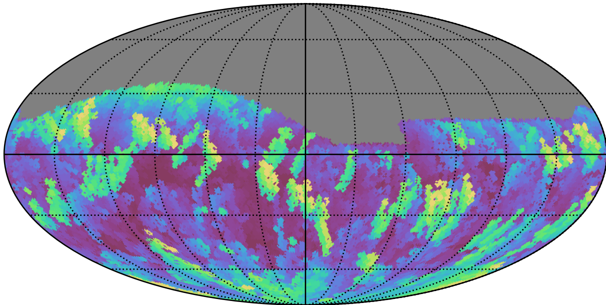
weather_cloudso0v3.5_10yrs Yr 1 i band: Max airmass
