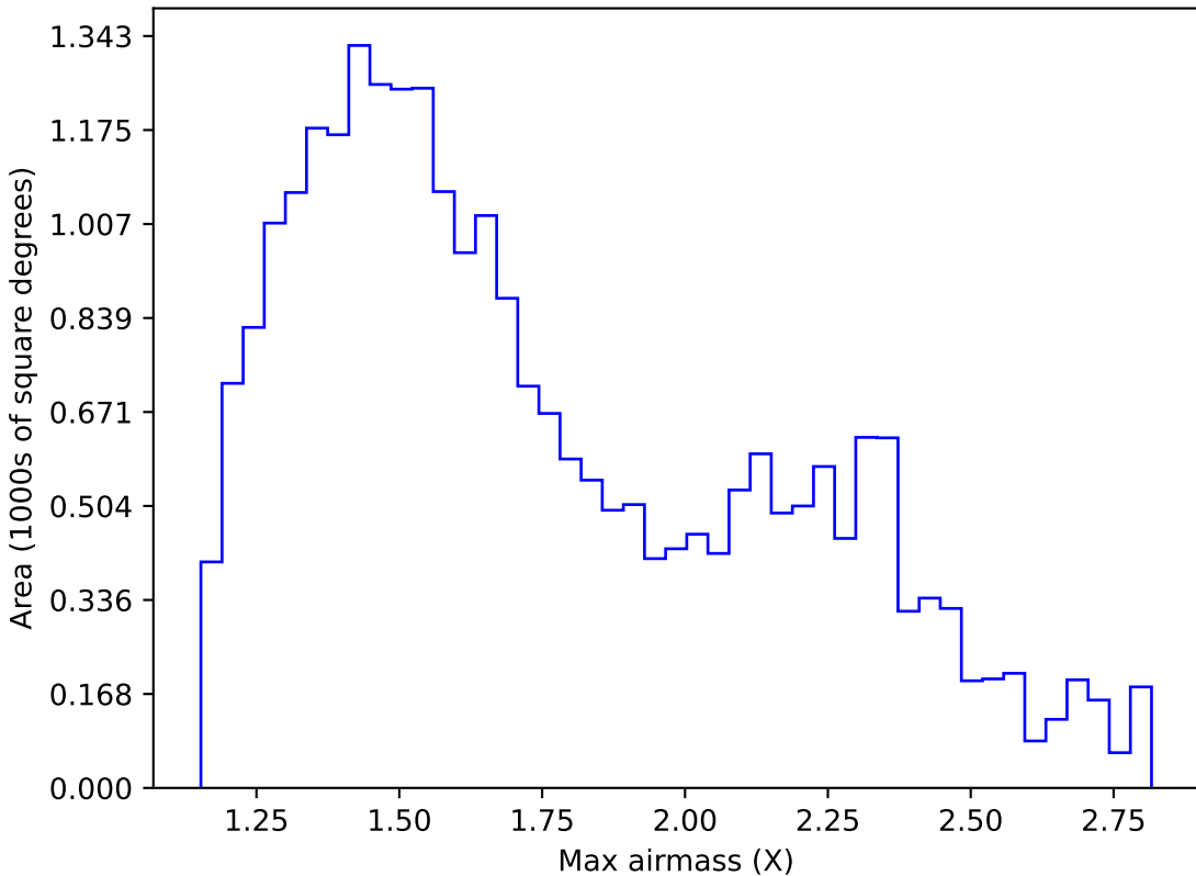
weather_cloudso0v3.5_10yrs Yr 1 i band: Max airmass
