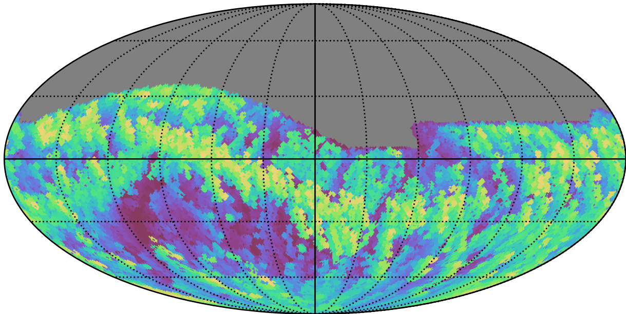
weather_cloudso0v3.5_10yrs Yr 1 all bands: Max airmass
