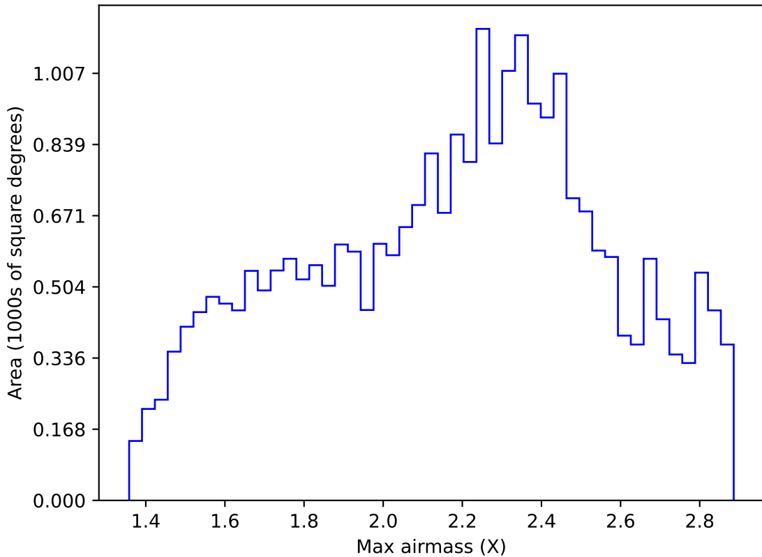
weather_cloudso0v3.5_10yrs Yr 1 all bands: Max airmass
