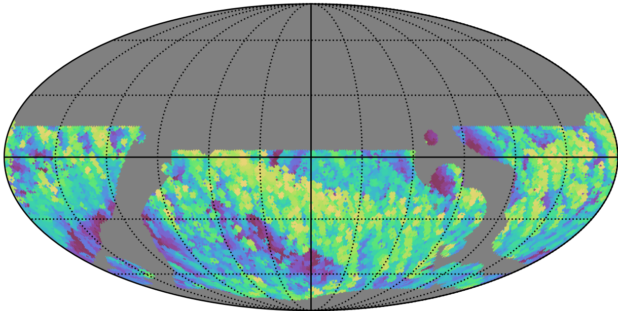
weather_cloudso0v3.5_10yrs WFD z band: Max airmass
