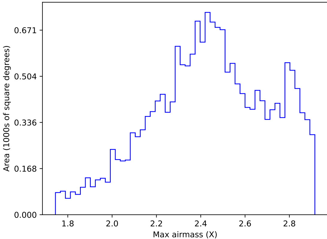
weather_cloudso0v3.5_10yrs WFD z band: Max airmass
