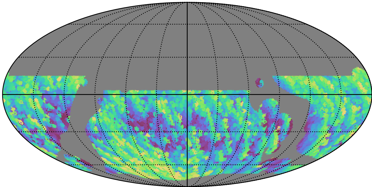
weather_cloudso0v3.5_10yrs WFD y band: Max airmass
