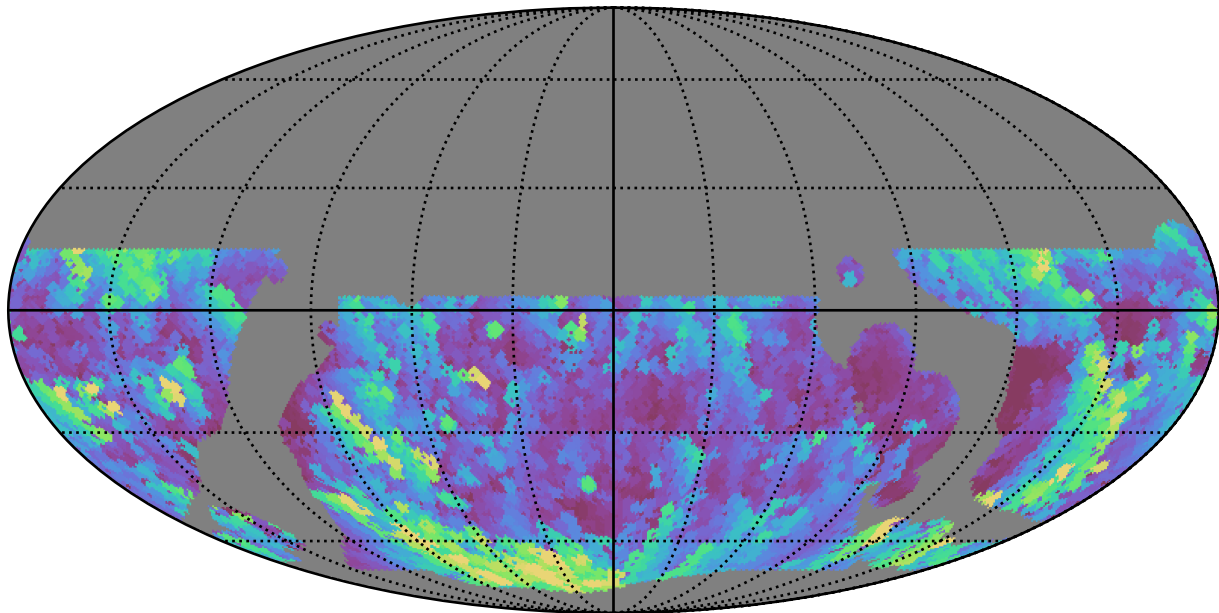
weather_cloudso0v3.5_10yrs WFD u band: Max airmass
