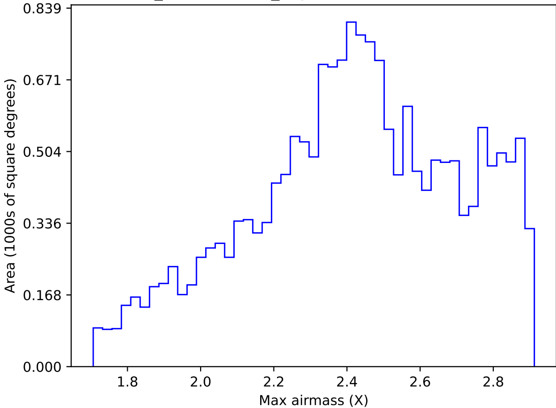
weather_cloudso0v3.5_10yrs WFD r band: Max airmass
