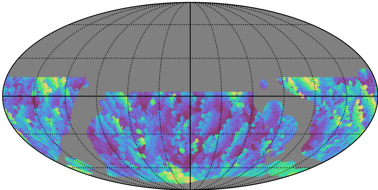
weather_cloudso0v3.5_10yrs WFD g band: Max airmass
