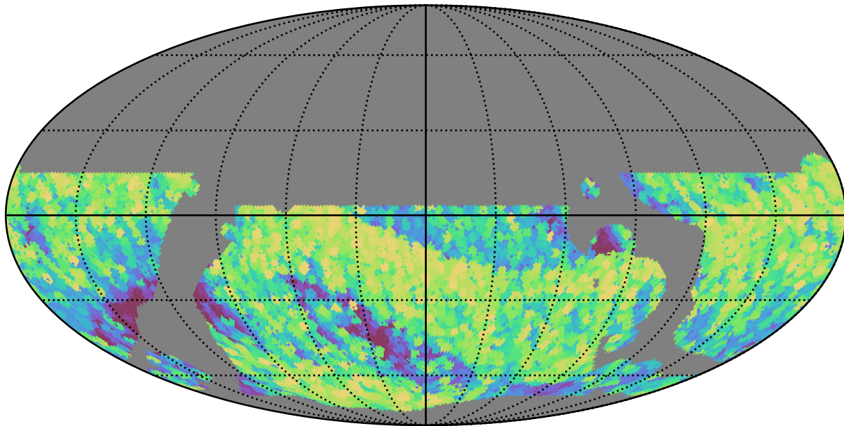
weather_cloudso0v3.5_10yrs WFD all bands: Max airmass
