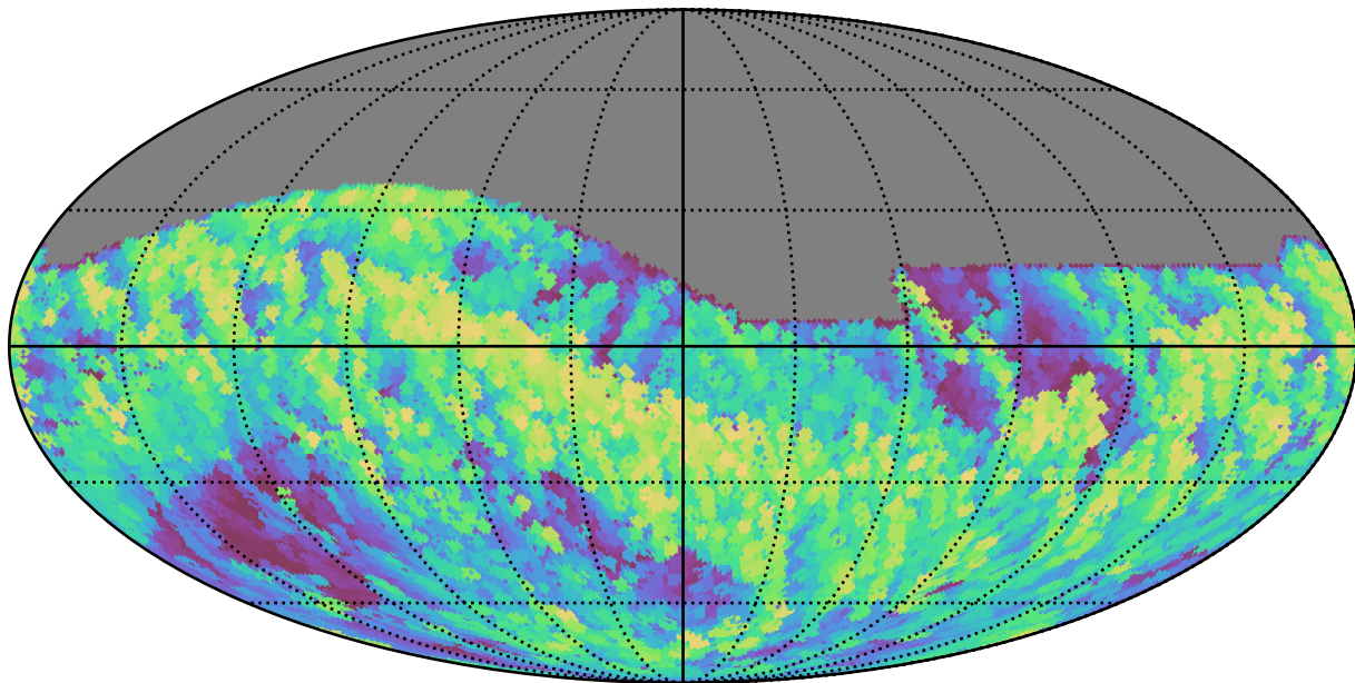
weather_cloudso0v3.5_10yrs All sky z band: Max airmass
