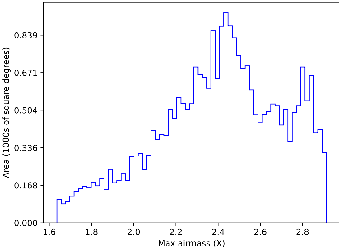
weather_cloudso0v3.5_10yrs All sky z band: Max airmass
