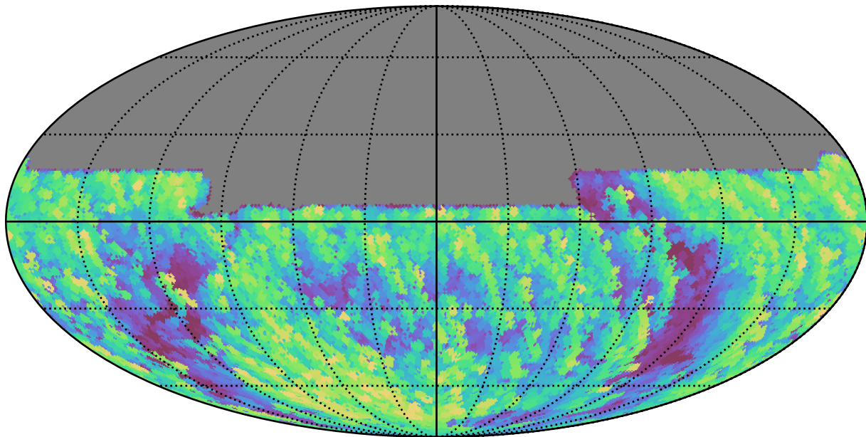
weather_cloudso0v3.5_10yrs All sky y band: Max airmass
