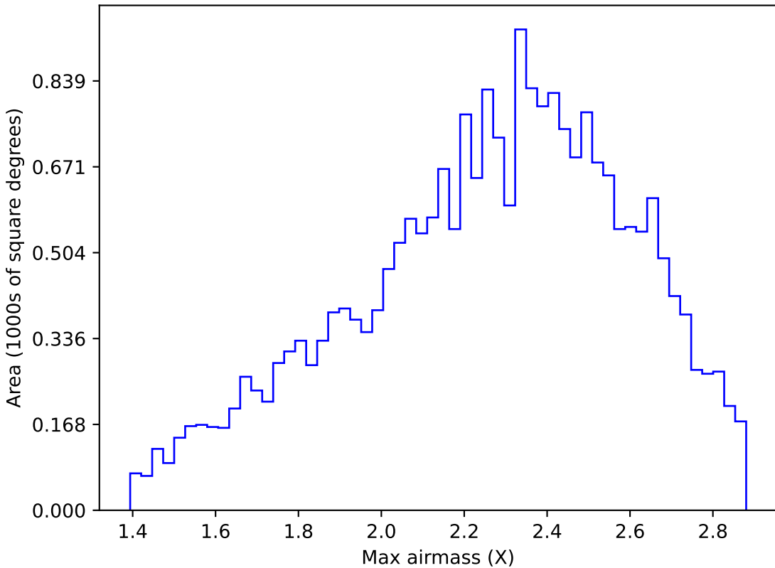
weather_cloudso0v3.5_10yrs All sky y band: Max airmass
