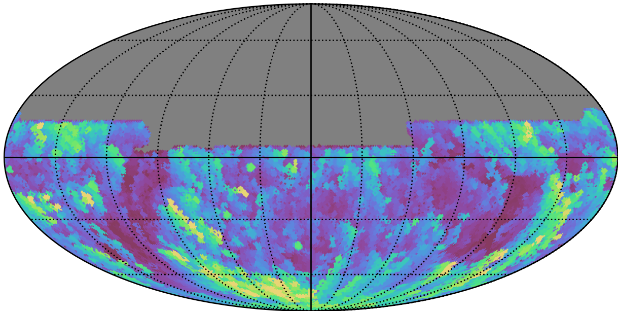
weather_cloudso0v3.5_10yrs All sky u band: Max airmass
