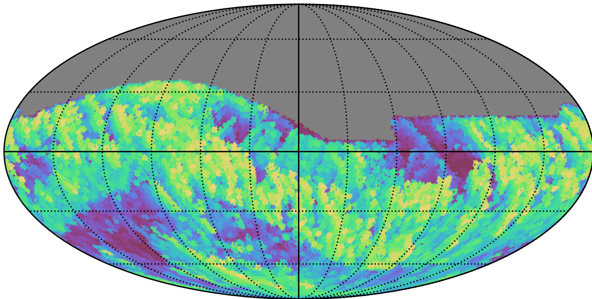
weather_cloudso0v3.5_10yrs All sky r band: Max airmass
