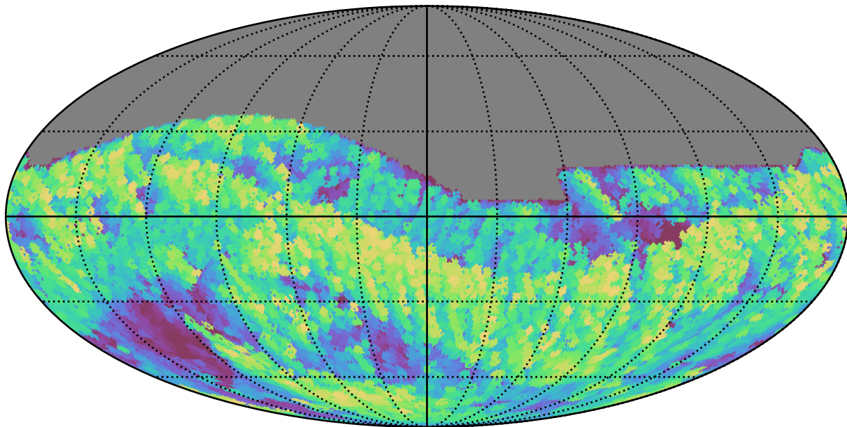
weather_cloudso0v3.5_10yrs All sky i band: Max airmass
