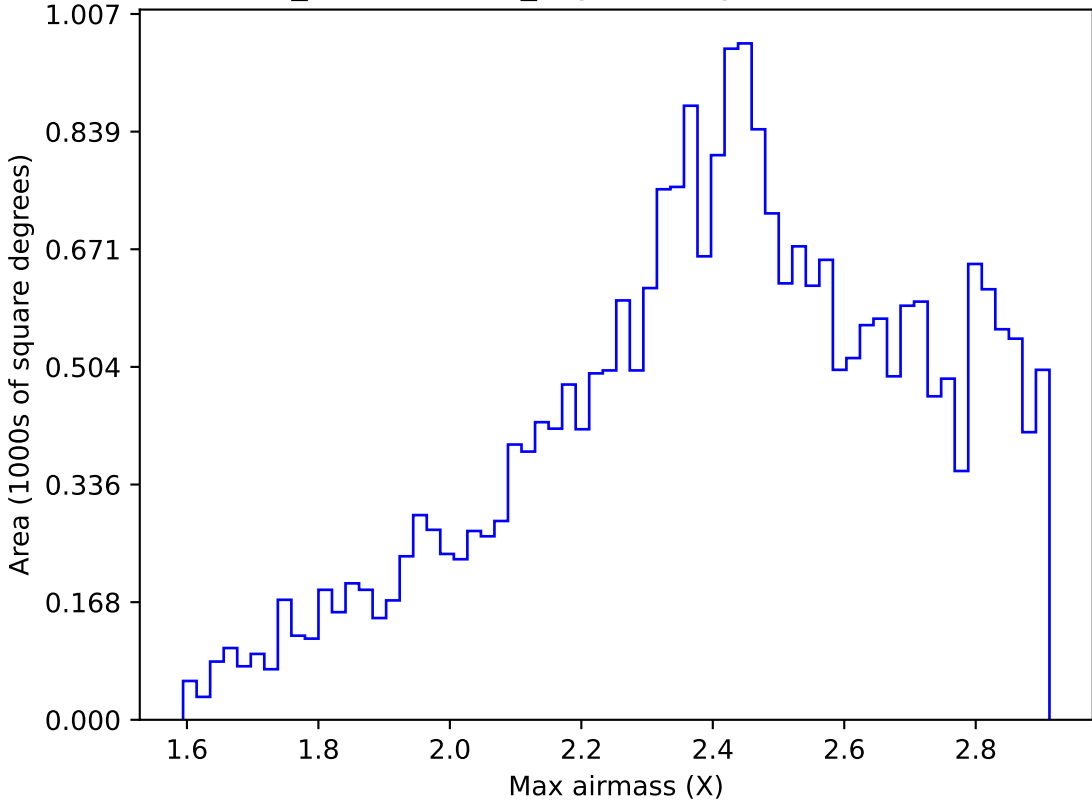
weather_cloudso0v3.5_10yrs All sky i band: Max airmass
