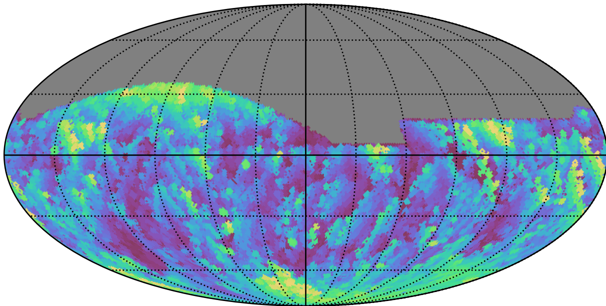
weather_cloudso0v3.5_10yrs All sky g band: Max airmass
