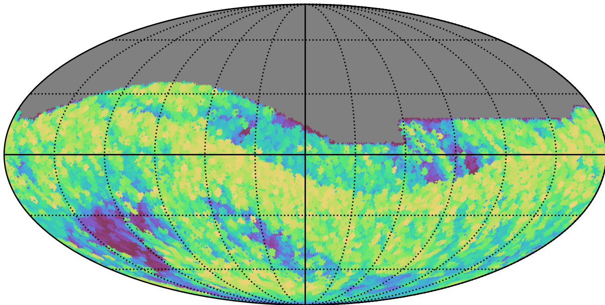
weather_cloudso0v3.5_10yrs All sky all bands: Max airmass
