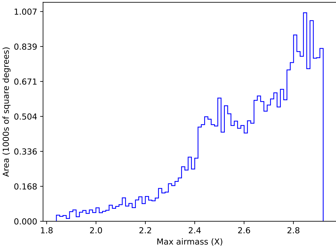
weather_cloudso0v3.5_10yrs All sky all bands: Max airmass
