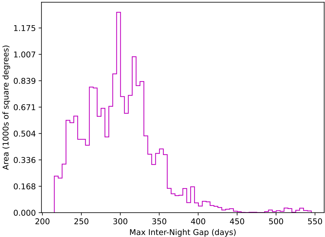
weather_cloudso0v3.5_10yrs WFD z band: Max Inter-Night Gap
