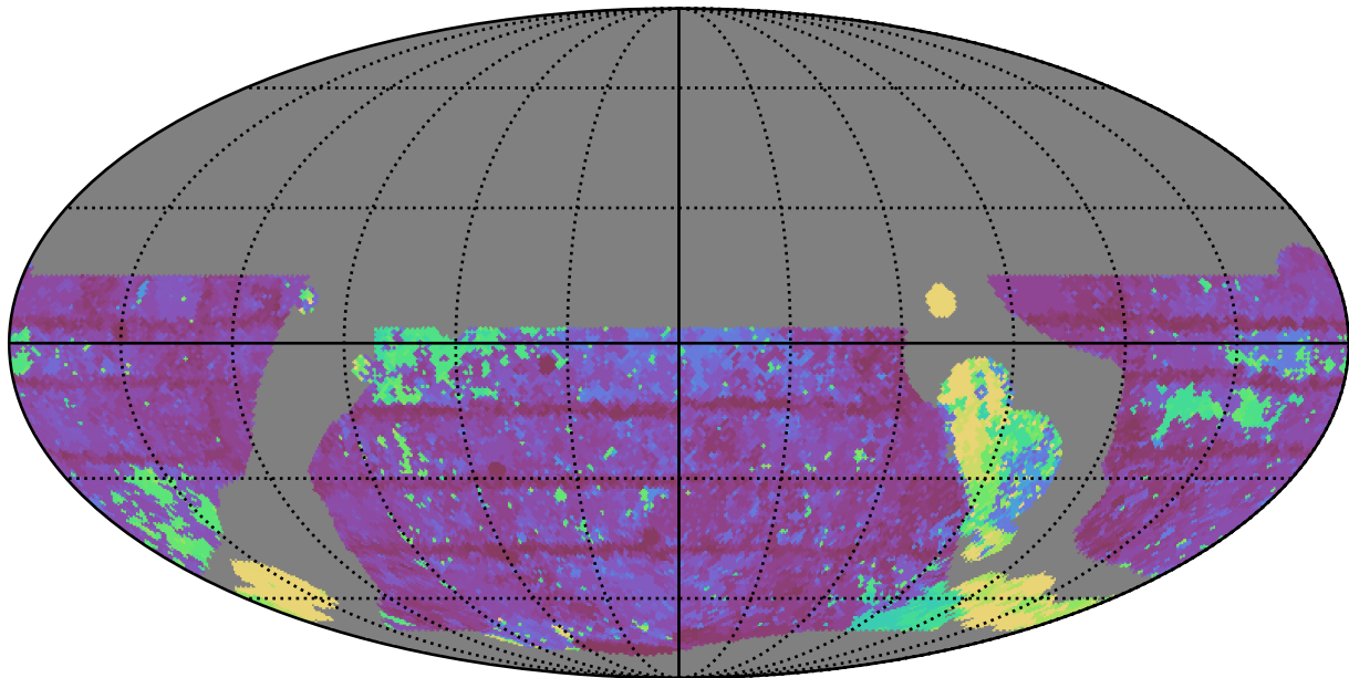
weather_cloudso0v3.5_10yrs WFD y band: Max Inter-Night Gap
