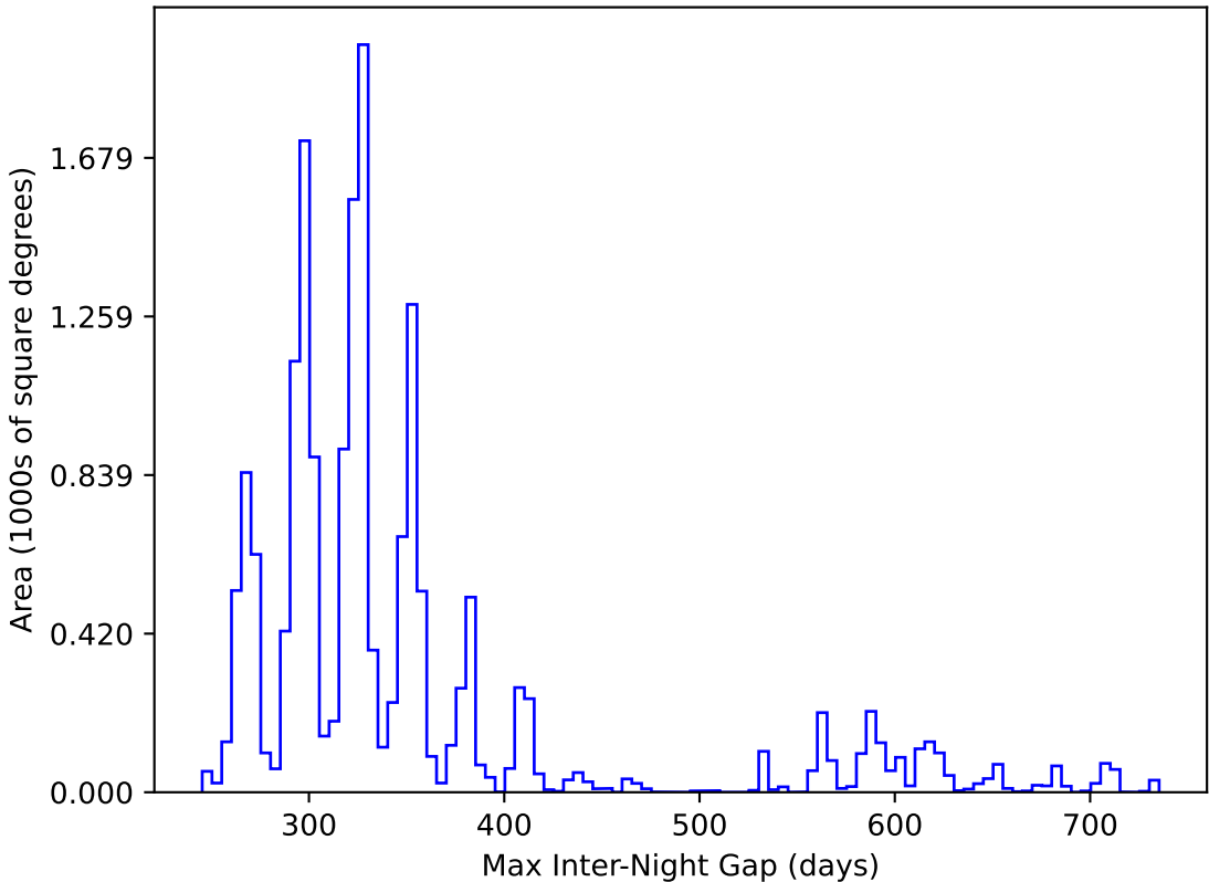
weather_cloudso0v3.5_10yrs WFD y band: Max Inter-Night Gap
