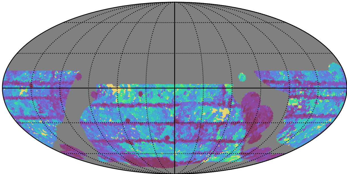
weather_cloudso0v3.5_10yrs WFD r band: Max Inter-Night Gap
