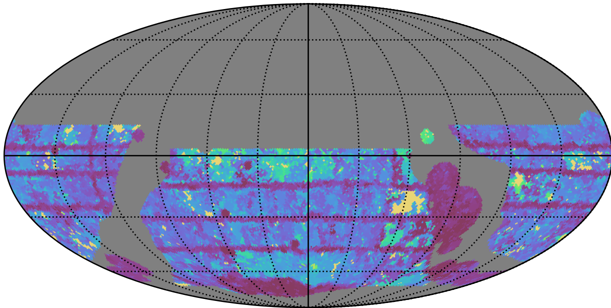
weather_cloudso0v3.5_10yrs WFD i band: Max Inter-Night Gap
