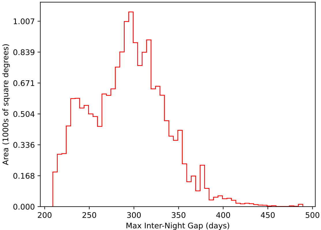
weather_cloudso0v3.5_10yrs WFD i band: Max Inter-Night Gap
