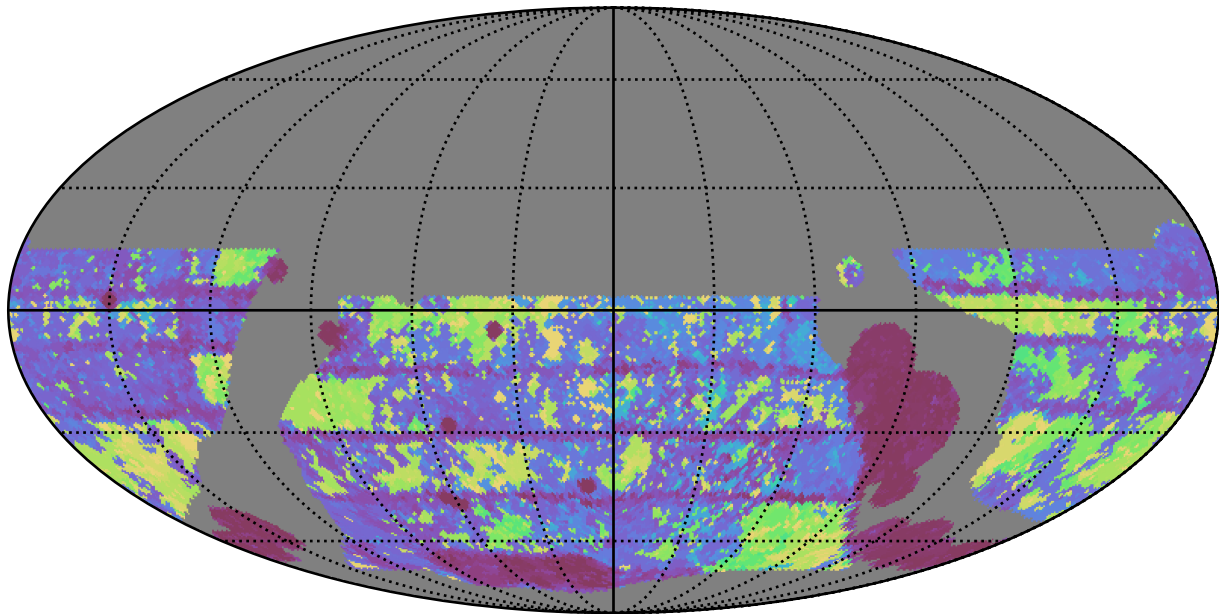
weather_cloudso0v3.5_10yrs WFD g band: Max Inter-Night Gap
