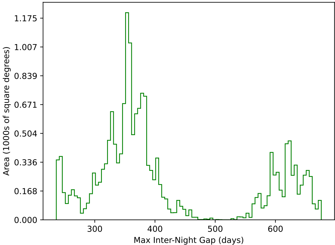
weather_cloudso0v3.5_10yrs WFD g band: Max Inter-Night Gap
