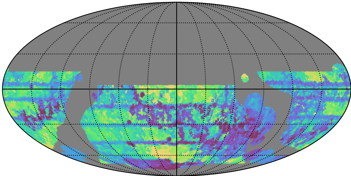
weather_cloudso0v3.5_10yrs WFD all bands: Max Inter-Night Gap
