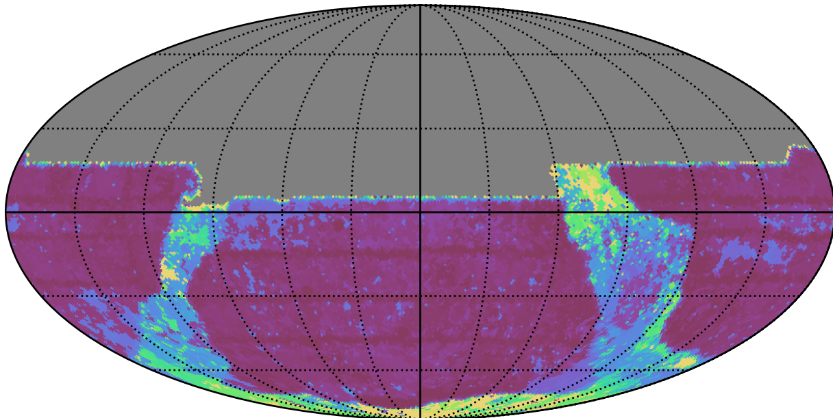
weather_cloudso0v3.5_10yrs All sky y band: Max Inter-Night Gap
