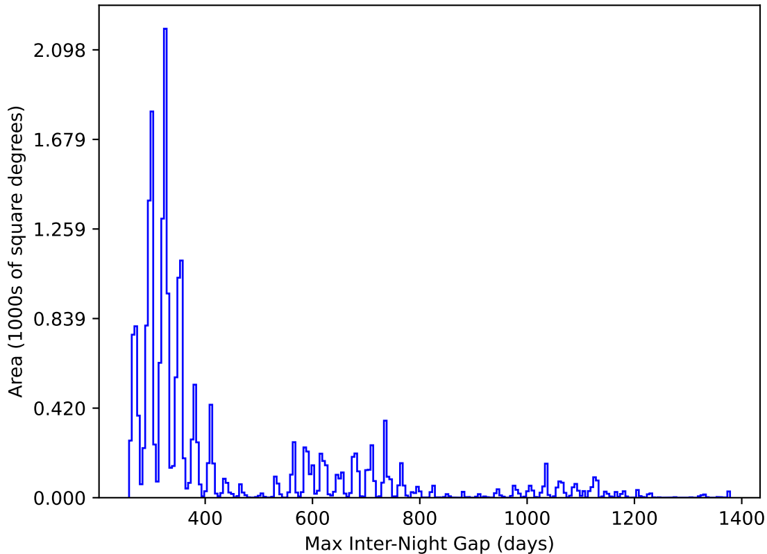
weather_cloudso0v3.5_10yrs All sky y band: Max Inter-Night Gap
