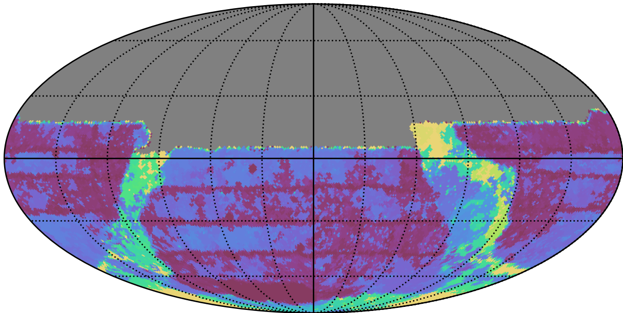
weather_cloudso0v3.5_10yrs All sky u band: Max Inter-Night Gap
