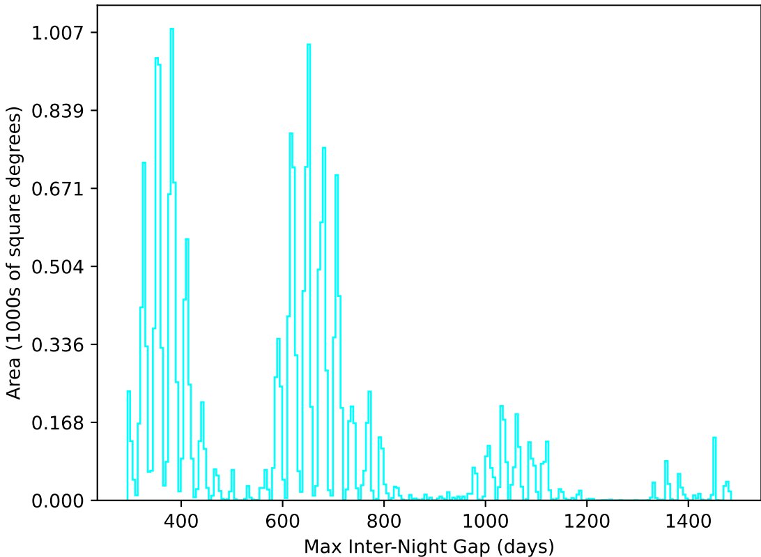
weather_cloudso0v3.5_10yrs All sky u band: Max Inter-Night Gap
