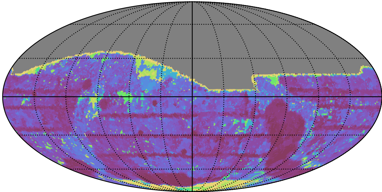
weather_cloudso0v3.5_10yrs All sky r band: Max Inter-Night Gap
