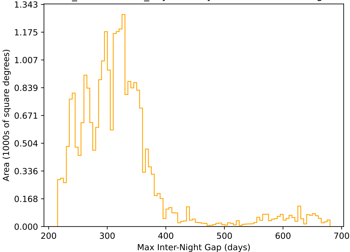
weather_cloudso0v3.5_10yrs All sky r band: Max Inter-Night Gap
