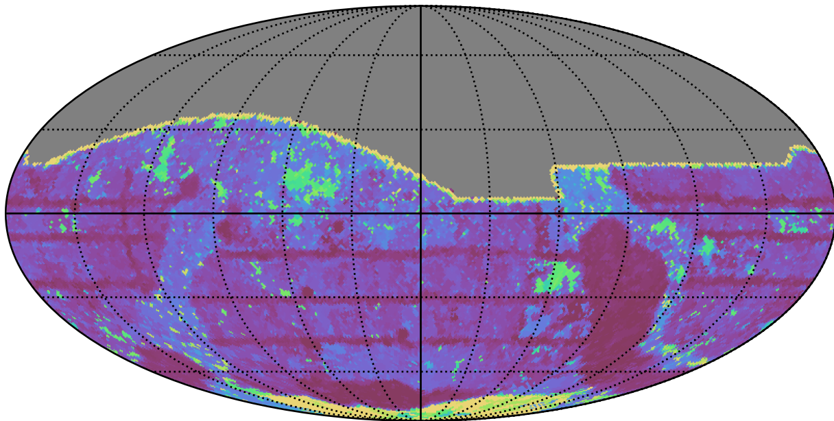
weather_cloudso0v3.5_10yrs All sky i band: Max Inter-Night Gap
