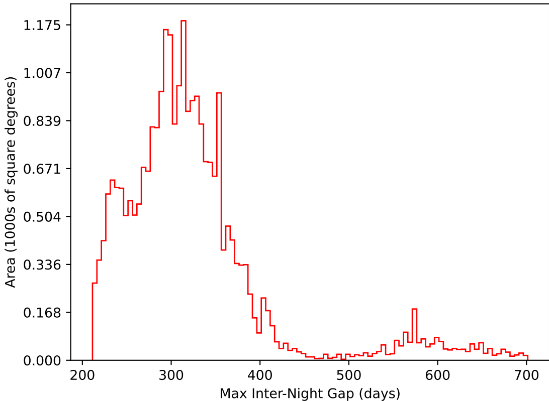
weather_cloudso0v3.5_10yrs All sky i band: Max Inter-Night Gap
