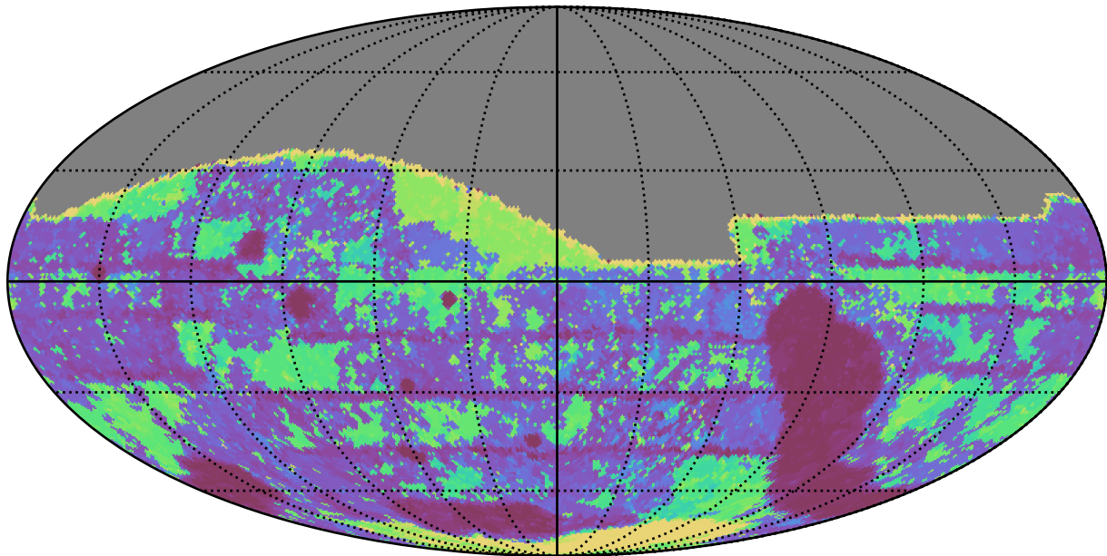
weather_cloudso0v3.5_10yrs All sky g band: Max Inter-Night Gap
