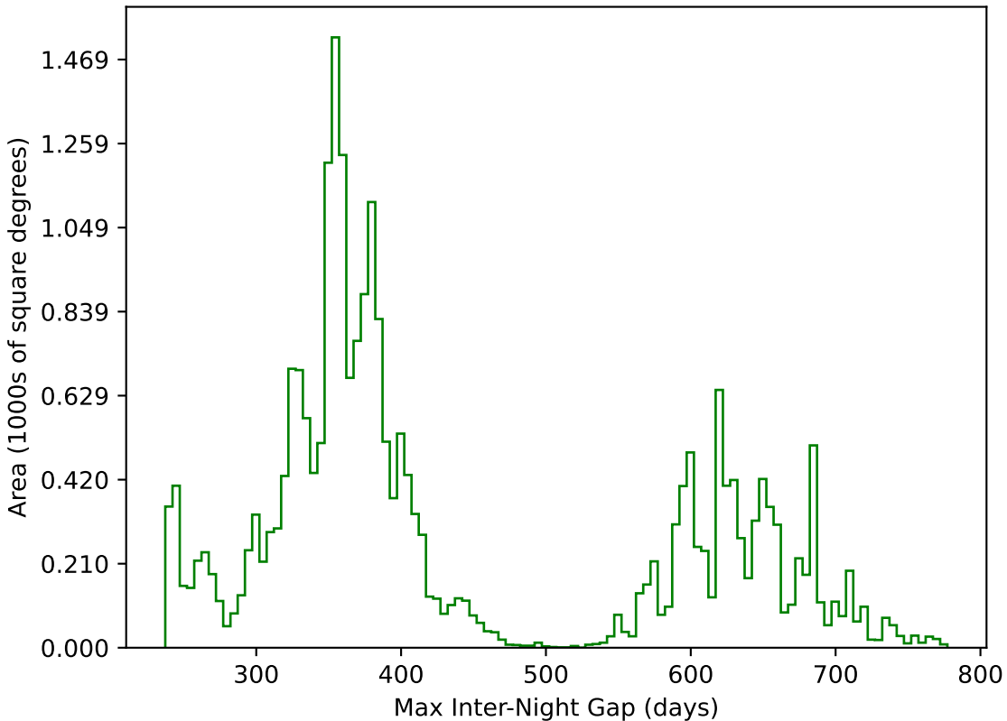
weather_cloudso0v3.5_10yrs All sky g band: Max Inter-Night Gap
