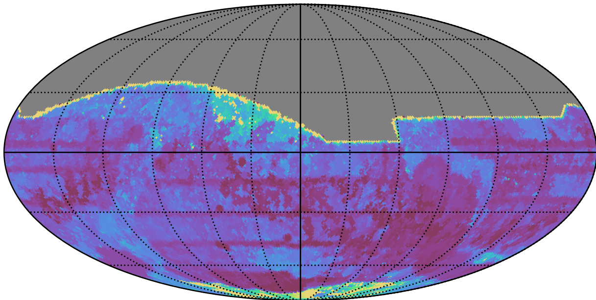
weather_cloudso0v3.5_10yrs All sky all bands: Max Inter-Night Gap
