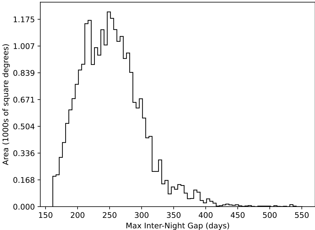
weather_cloudso0v3.5_10yrs All sky all bands: Max Inter-Night Gap
