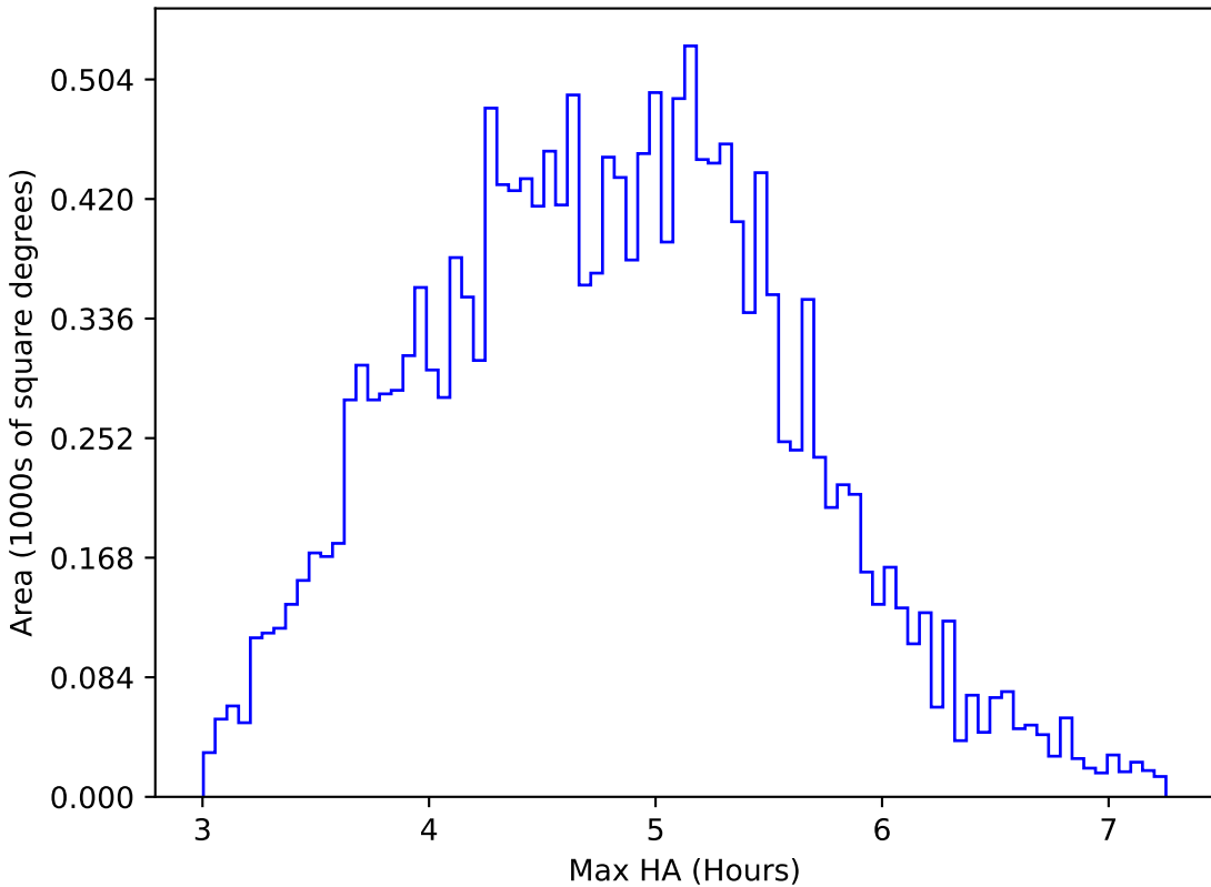
weather_cloudso0v3.5_10yrs WFD z band: Max HA
