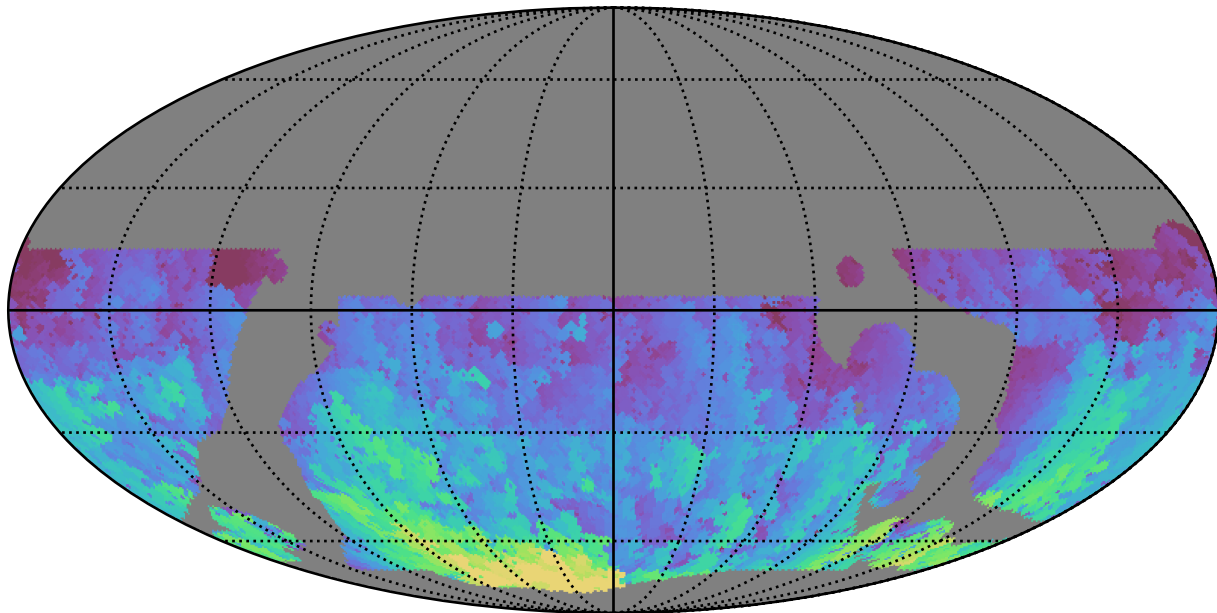
weather_cloudso0v3.5_10yrs WFD u band: Max HA
