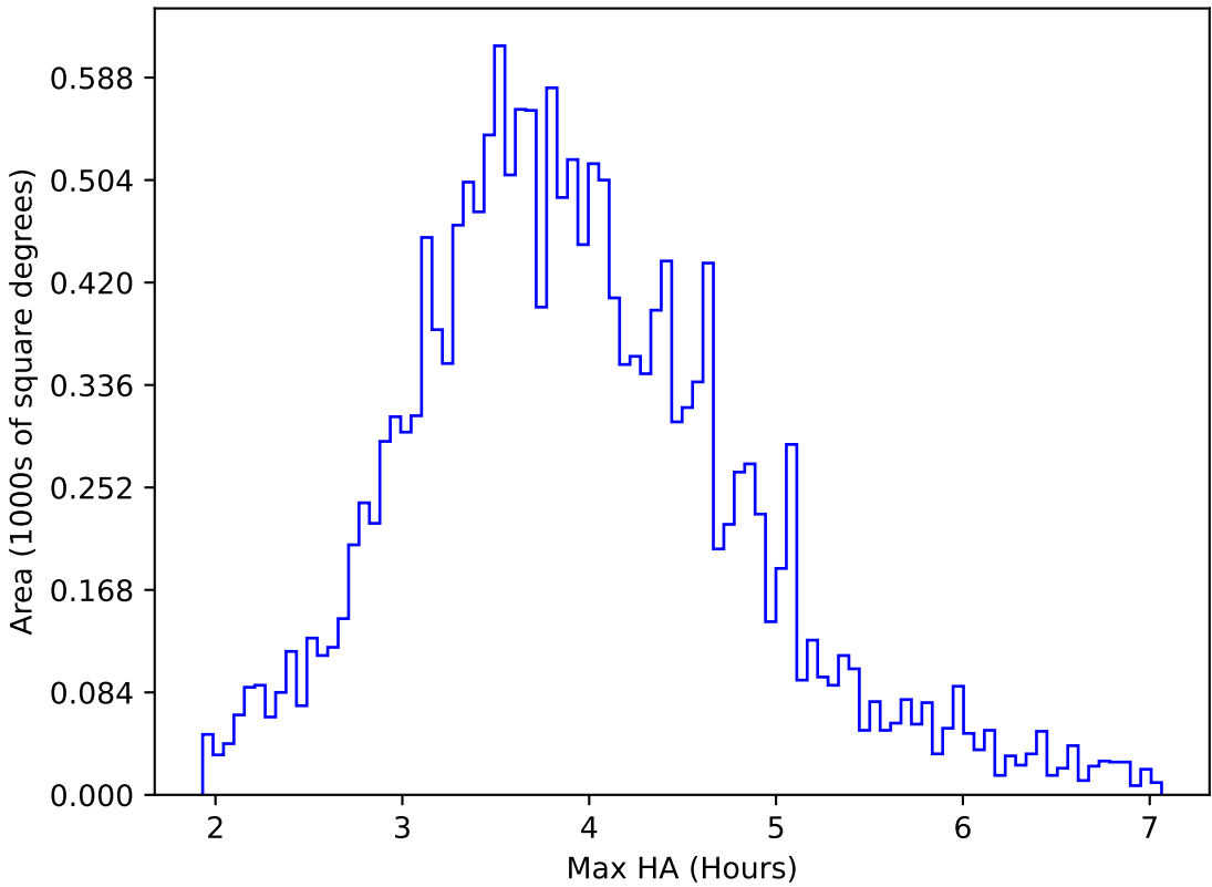
weather_cloudso0v3.5_10yrs WFD u band: Max HA
